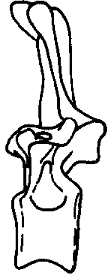
lateral view
