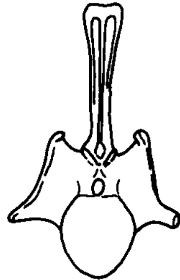
rear view
